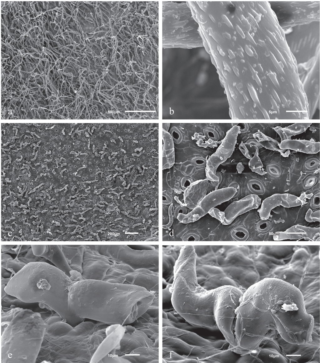
Fig. 8: Diospyros ketun (a–b): a: abaxial leaf surface with long, flexuose hairs; – b: hair with warts and longitudinal elevations on hair surface (a–b from Martinelli & Távora 2709 [W]); – D. mexiae (c–f): indumentum, 2-armed hairs and stomata (c–f from Mexia 4316, isotype [PH]); – (SEM-photographs: Wencke Wegner, Central Research Laboratories, Natural History Museum Vienna).
