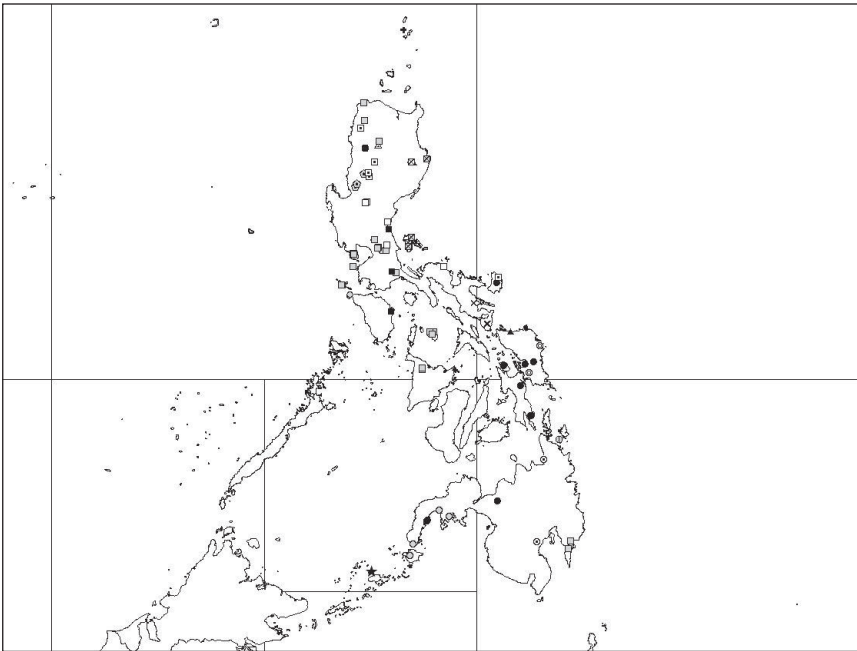
Fig. 5. Distributions of species endemic to the Philippines. Most species have narrow distributions (each species is signified by a different symbol), the exception being C. micrantha (grey squares). The Geunsia group of species are restricted to the southern islands (circular symbols).
