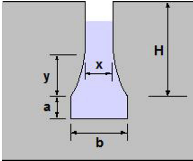
Figure 5.2.5.6 Weir Dimensions
