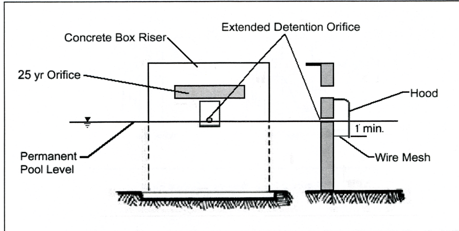
Figure 5-10 Hooded Outlet
