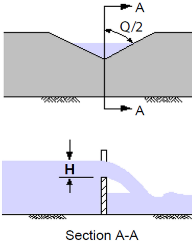
Figure 5.2.5.5 V-Notch Weir
