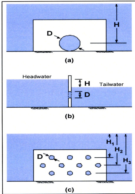
Figure 5-1 Orifice Definitions
