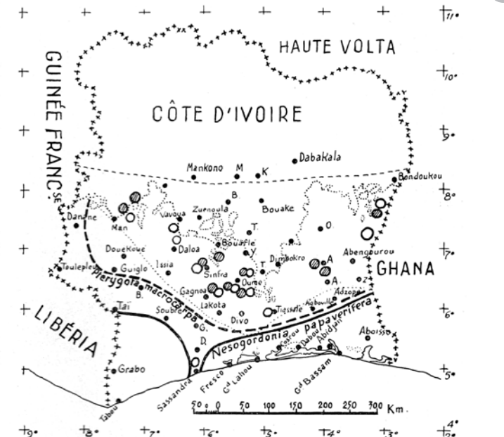
..... Boundary of dense humid forest ..... Patches of humid forest in savannah or of savannah in dense forest ----- Northern limit of the pre-forest zone ..... Boundary between semi-deciduous Malva and Ulmaceae forest and evergreen forests with leguminous species ○ Very abundant Nesogordonia papaverifera (kotibé) ○ Pterygota macrocarpa (Koto)
