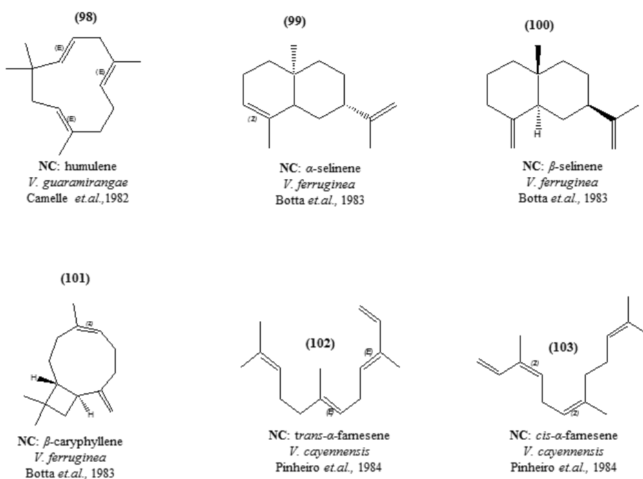
Fig. 7.21 Sesquiterpenes isolated from several Vismia species.
