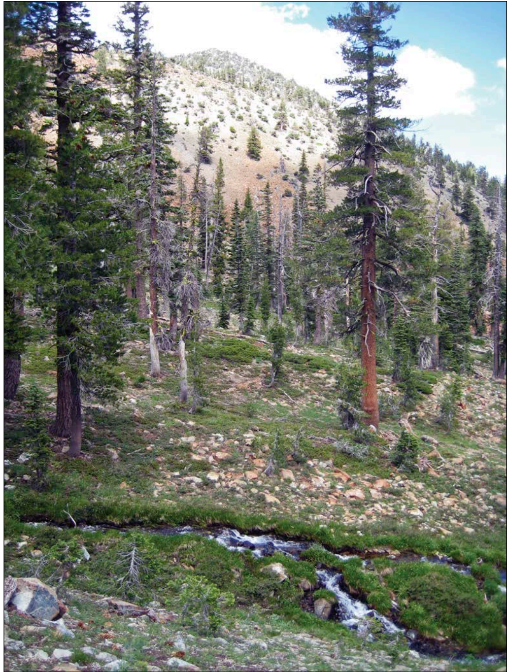
Figure 3.2—Red fir and western white pine growing on ultramafic soils near Mount Eddy, Shasta-Trinity National Forest; elevation 2180 m.
