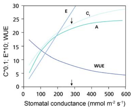
FIGURE 28. The effect of stomatal conductance ( g_s ) on the transpiration rate ( E , \text{mmol m}^{-2} \text{s}^{-1} ), rate of \text{CO}_2 assimilation ( A , \mu\text{mol m}^{-2} \text{s}^{-1} ), intercellular \text{CO}_2 concentration ( C_i , \mu\text{mol mol}^{-1} ) and photosynthetic water-use efficiency (WUE, \text{mmol CO}_2 (\text{mol H}_2\text{O})^{-1} \text{s}^{-1} ) as a function of stomatal conductance. Calculations were made assuming a constant leaf temperature of 25^\circ\text{C} and a negligible boundary layer resistance. The arrow indicates g_s at the co-limitation point of carboxylation and electron transport. For the calculations, Equations as described in Box 2A.1 and Sect. 2.2.2 have been used.
