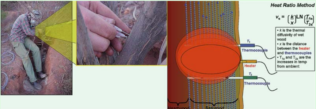
FIGURE 1. Sap-flow measurements using the heat-ratio method require insertion of probes in a stem, root, or branch (left). The middle probe is a heater, the other ones are thermocouples. If sap moves upward, then the heat pulse will reach the upper
