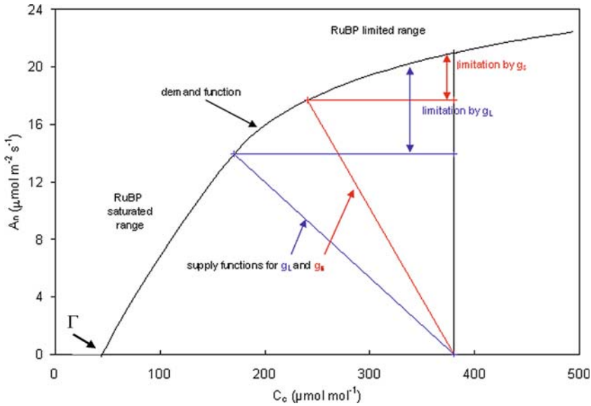
FIGURE 6. The relationship between the rate of net \text{CO}_2 assimilation ( A_n ) and the \text{CO}_2 concentration at the site of Rubisco in the chloroplasts ( C_c ) for a \text{C}_3 leaf: the “demand function”. The concentration at which A_n = 0 is the \text{CO}_2 -compensation point ( \Gamma ). The rate of diffusion of \text{CO}_2 from the atmosphere to the intercellular spaces and to Rubisco in the chloroplast is given by the “supply functions” (the red and blue lines). The slopes of these lines are the leaf conductance ( g_L ) and mesophyll
