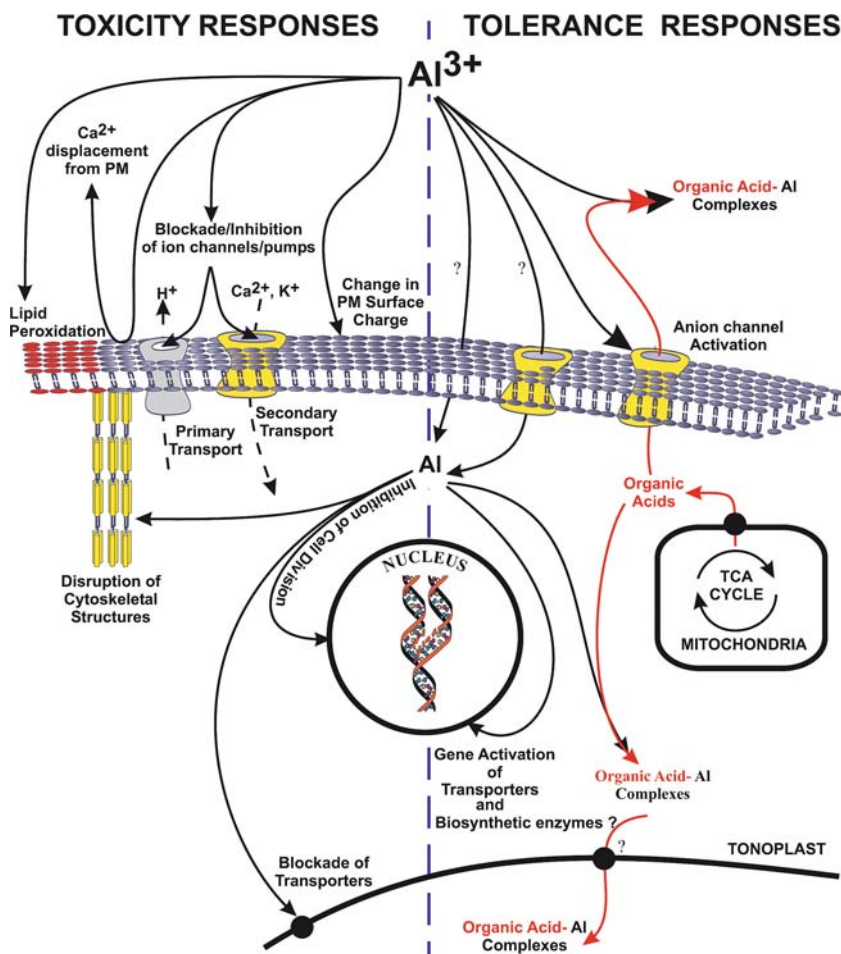
FIGURE 22. Possible mechanisms of Al toxicity and Al resistance in plants. Al toxicity targets are illustrated on the left side of the diagram. For clarity, the interactions of Al with the cell wall are not shown. On the right side, Al-resistance mechanisms (Al exclusion and internal Al detoxification) are based on the formation of Al complexes with
