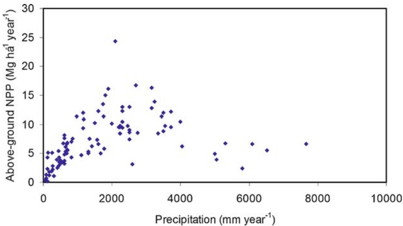
FIGURE 1. Correlation of above-ground net primary production (NPP, in units of biomass) with precipitation. NPP declines at extremely high precipitation ( >3 \text{ m yr}^{-1} ) due to indirect effects of excess moisture, such as low soil oxygen and nutrient loss by leaching (Schoor 2003). Copyright Ecological Society of America.
