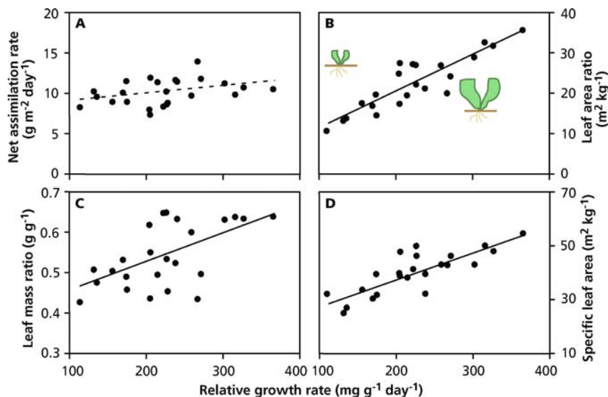
FIGURE 3. A comparison of the NAR, LAR, LMR, and SLA of 24 herbaceous C_3 species that differ in their RGR as determined on plants grown with free access to
