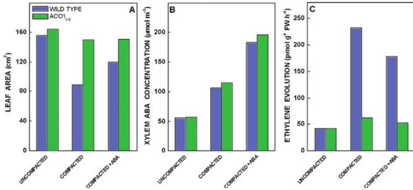
FIGURE 17. Effects of soil compaction on leaf growth, xylem ABA concentration, and ethylene production in wild type and a transgenic with a low capacity to produce ethylene of Solanum lycopersicum (tomato). (A) Total leaf area; (B) xylem sap ABA concentration; (C) leaf ethylene evolution at 21 days after emergence. Plants were well watered and grown in a split-pot
