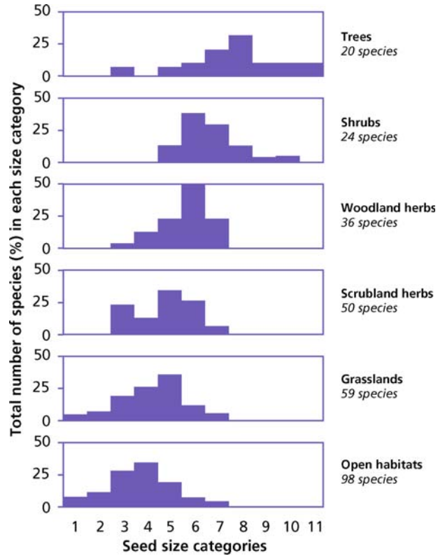
FIGURE 14. Frequency distribution of seed size in different ecological groups of plants (after Salisbury 1942). Species that establish in closed habitats tend to have larger seeds than open-habitat plants.
