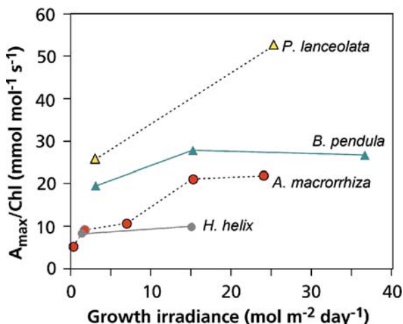
FIGURE 14. Light-saturated rate of CO 2 assimilation ( A_{\max} ) per unit chlorophyll in relation to growth irradiance for four different species. Plantago lanceolata (snake plantain) (Poot et al. 1996), Betula pendula (European white birch, Bp) (Öquist et al. 1982), Alocasia macrorrhiza (giant taro, Am) (Sims & Pearcy 1989), Hedera helix (ivy, Hh) (T.L. Pons, unpublished data).
