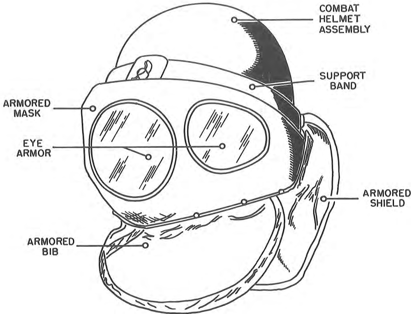
FIG. 8 MINE CLEARANCE PROTECTIVE ASSEMBLY FOR HEAD, FACE AND NECK.
