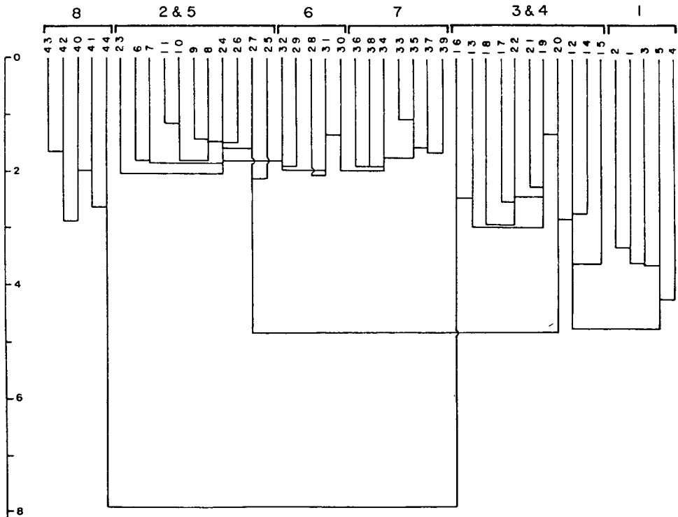
Fig. 17. Nearest-neighbour phenogram generated from the Manhattan distance matrix of the 44 specimens of the P. laricoides complex (based on all characters except KHDJ). Population numbers (as used in Table 11 and Fig. 34) are given above the brackets. The numbers directly above the phenogram refer to the specimens (refer Table 12 for details of collectors and collection numbers).
