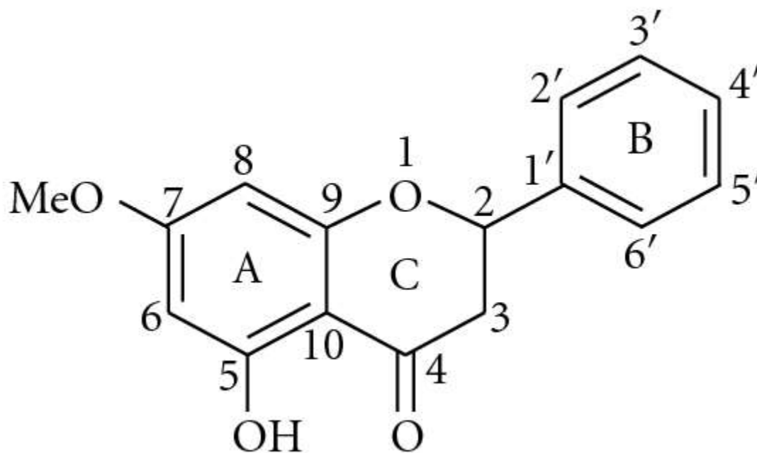
Figure 2 Structure of pinostrobin.
