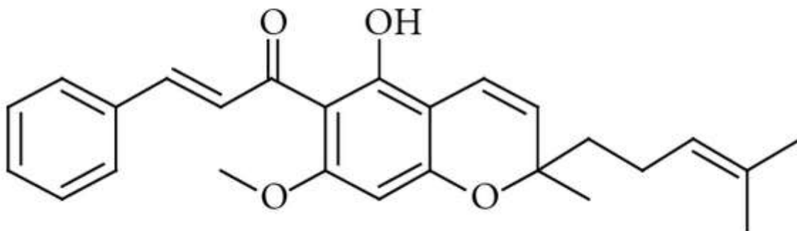
Figure 3 Structure of boesenbergin B.
