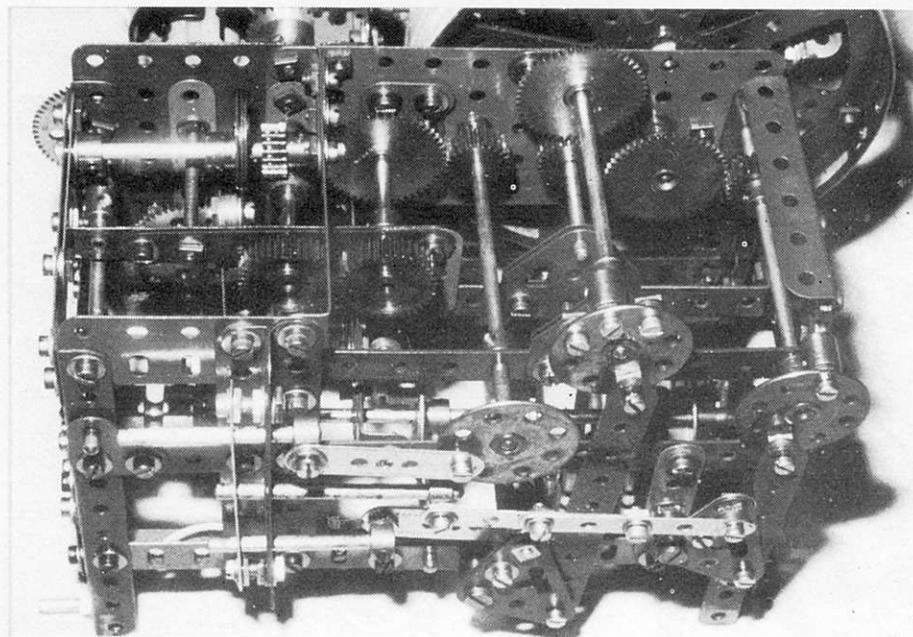
A detail illustration of the business end of the Author's Fruit Machine model, showing good use of 'double' bearings and washers.
