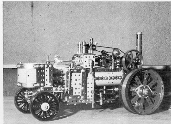
Below: A finely detailed model of an unusual subject, a Suffolk Punch Agricultural Engine built by Barry Wilkinson of the NEMS.
