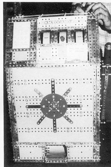
Operator's-eye view of the Author's Fruit Machine. Using modular construction techniques and employing over 300 washers for spacing purposes alone, it reproduced every feature of its prototype.
