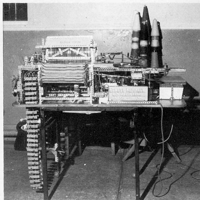
Ernest Keighley of Preston amazed all who watched the fascinating motions of his improved, automatically operating Rapier Loom.
