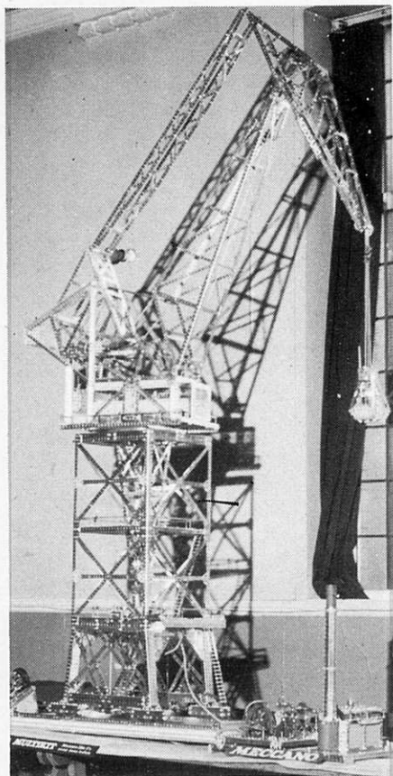
Left: Chris Barron, Chairman of the North Eastern Meccano Society, showed this superb Toplis Level Luffing Crane, over six feet tall. No less than five Power Drive Units are incorporated.
