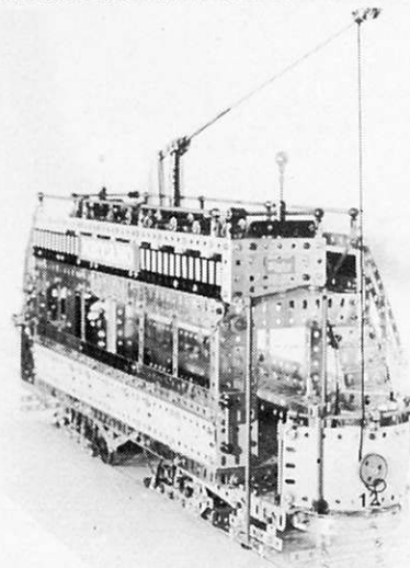
Stairway, handrails, trolley pole and many other fine details are evident in this end view of the Tramcar. Models of this type are ideal for Exhibition work, where their fine detailing can be displayed to the best advantage.
