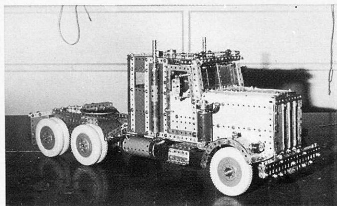
Top-Class modelling skill is clearly evident in this Kenworth Truck Unit by Keith McCallum. The scale proportions and wealth of detail add to the impression of realism.
