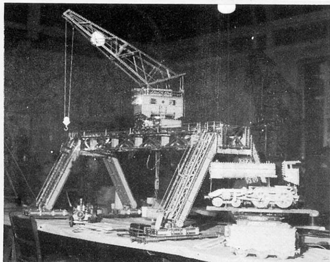
Mike Cotterill's stupendous Dockyard Gantry Crane displayed his usual high standard of modelling skill. Standing nearly six feet high and drawing power from seven motors, it took first prize in the adults' section of the model building competition.
